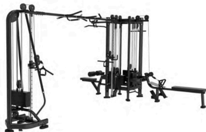
TB94 MULTI-JUNGLE(5 STATION) Weight:1350kg Size:5600×2700×2550mm PackingSize:2560×770×750mm/2420×1120×920mm Weight Stack:80kg×2/100kg×3
